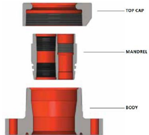
MODEL "GT-6"
